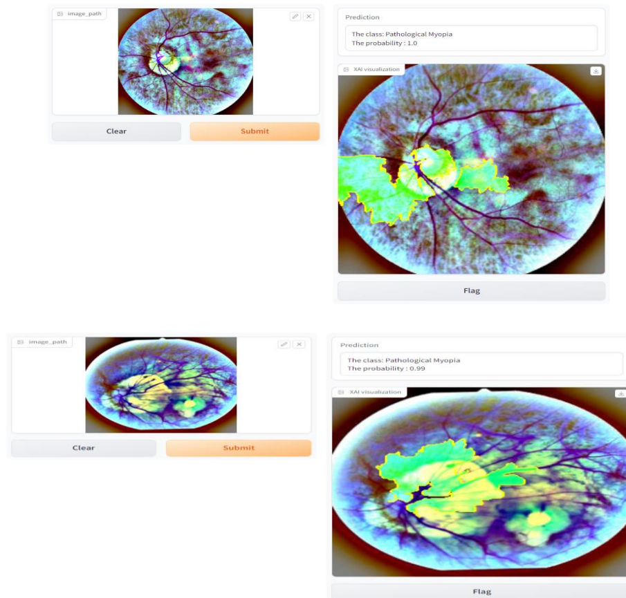
Fig. 11. User interface for myopia detection with XAI model (two random myopia cases)
