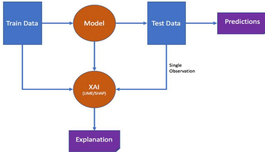
Fig. 6. LIME architecture [25]
