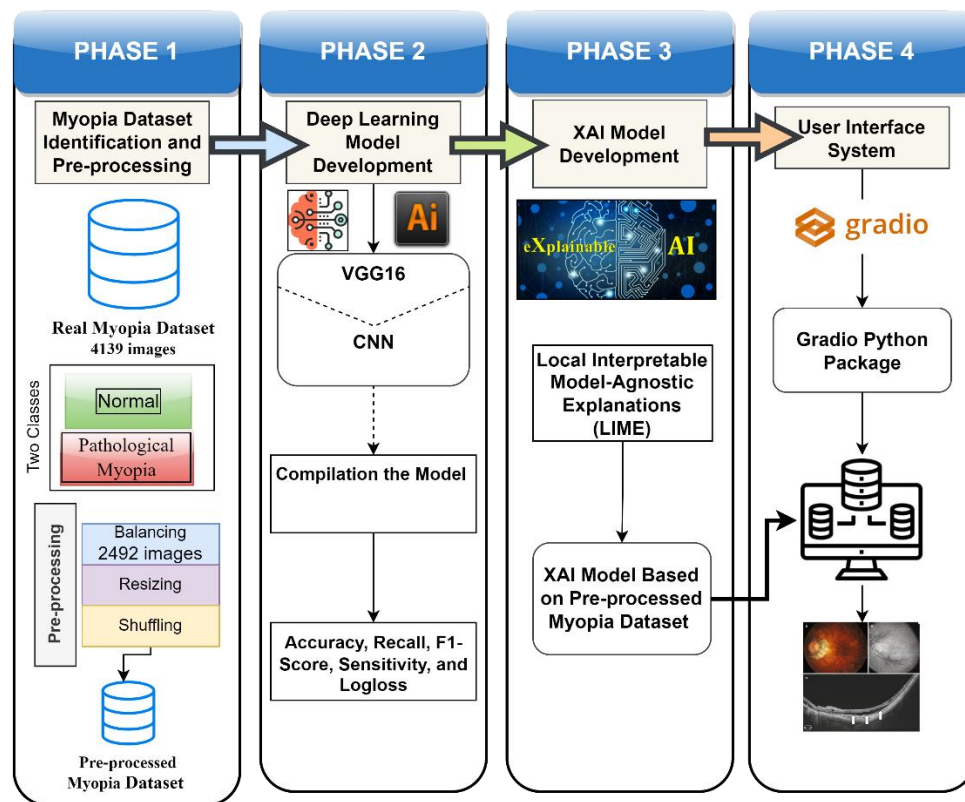
Fig. 1. Integration methodology phases for myopia detection
