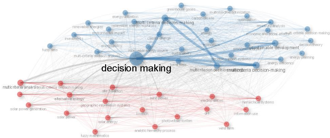
Fig. 5. Co-Occurrence Network
