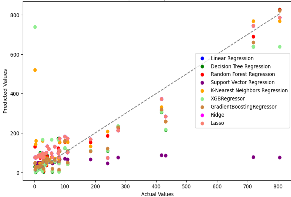
Fig. 13. Relationships between actual and predicted values across various regression models
