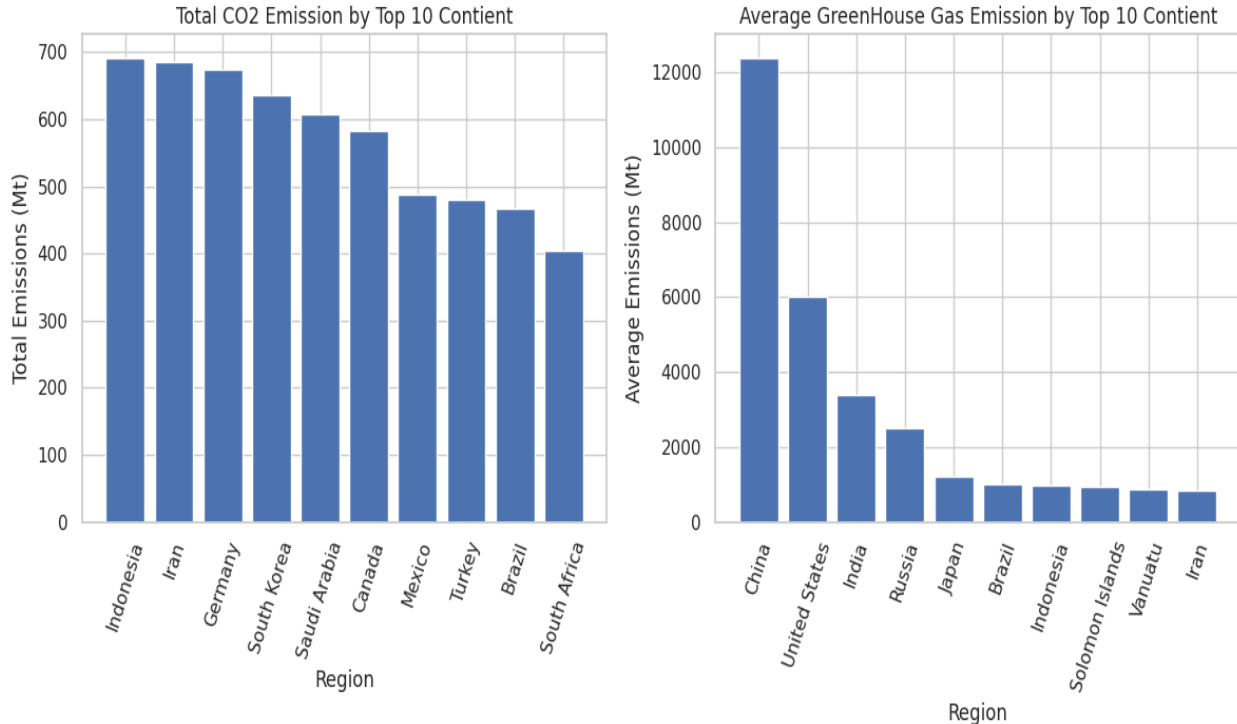
Fig. 12. Comparative analysis of CO2 emissions and average greenhouse gas emissions across the top emitters
