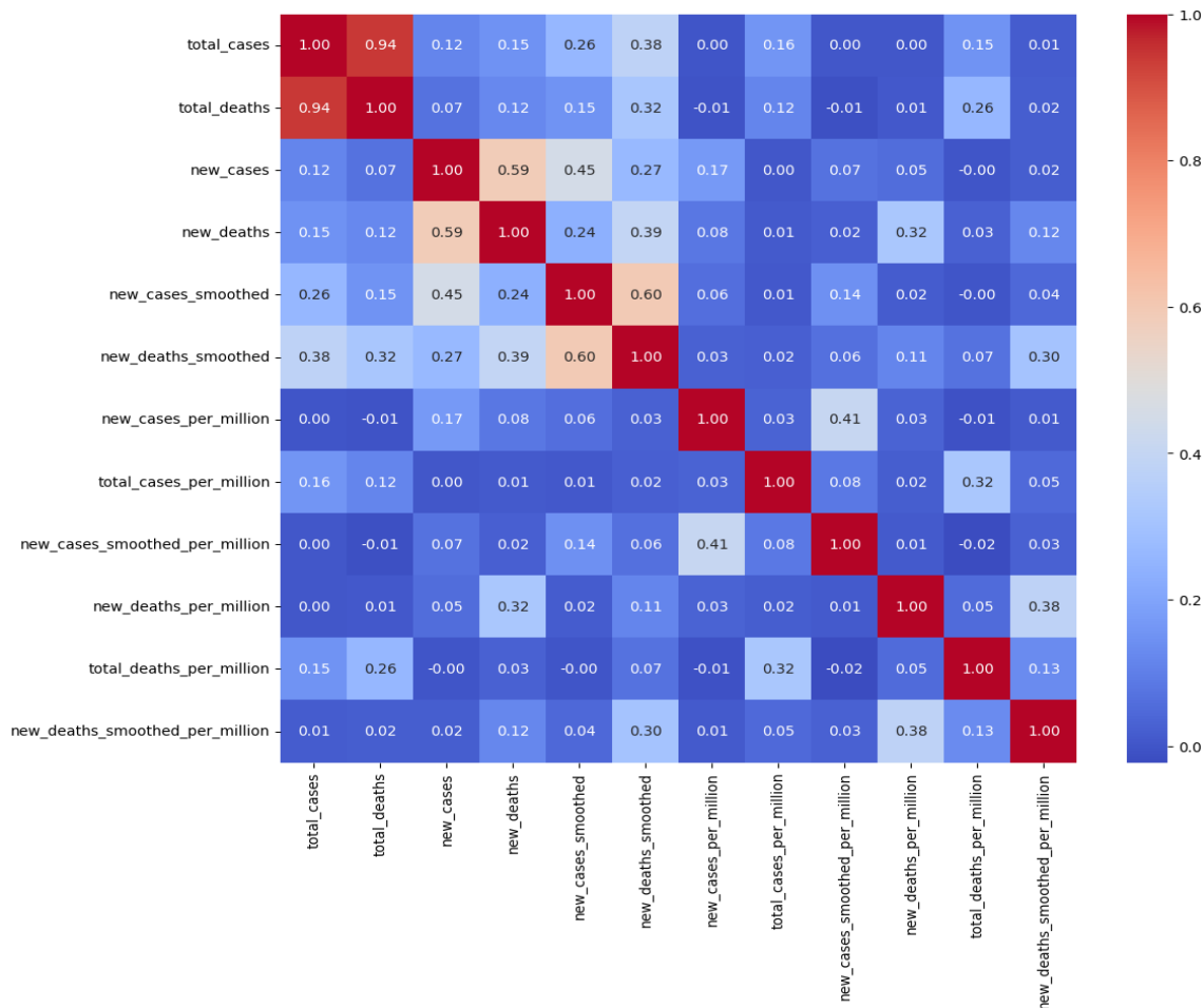
Fig. 8. Correlation matrix
