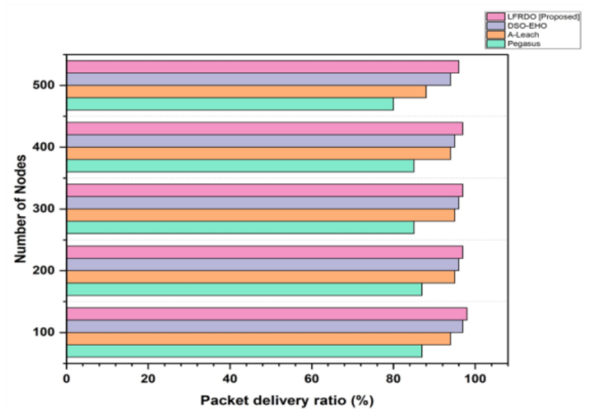
Fig. 4. Results of Packet delivery ratio
