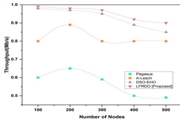
Fig. 6. Throughput's comparison
