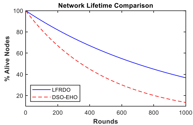
Fig. 7. Network Lifetime Comparison
