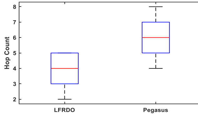
Fig. 9. . Path Optimality Comparison
