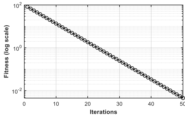
Fig. 10. LFRDO convergence rate
