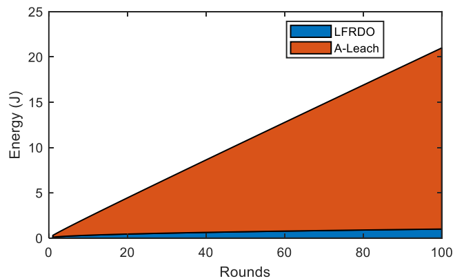
Fig. 8. Cumulative energy consumption
