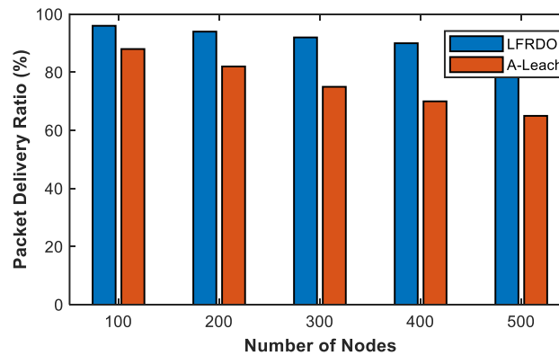
Fig. 11. Scalability: PDR vs. network size
