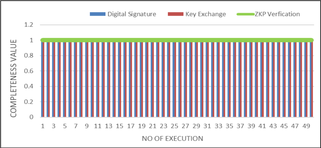
Fig.16. Completeness measure for QESM system operations.
