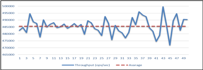
Fig.17. QESM system throughput.
