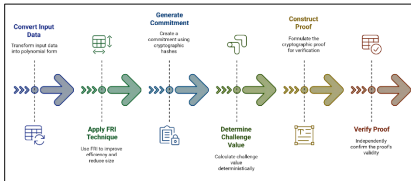
Fig. 4. NIZK-STARKs verification process.
