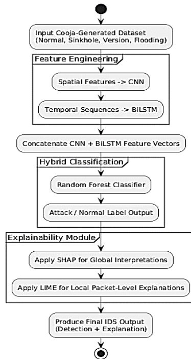
Fig. 5. Hybrid AI-Driven IDS Architecture with CNN–BiLSTM–RF and XAI Integration
