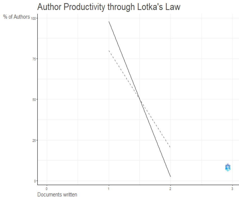
Fig. 5. Lotk's Law
