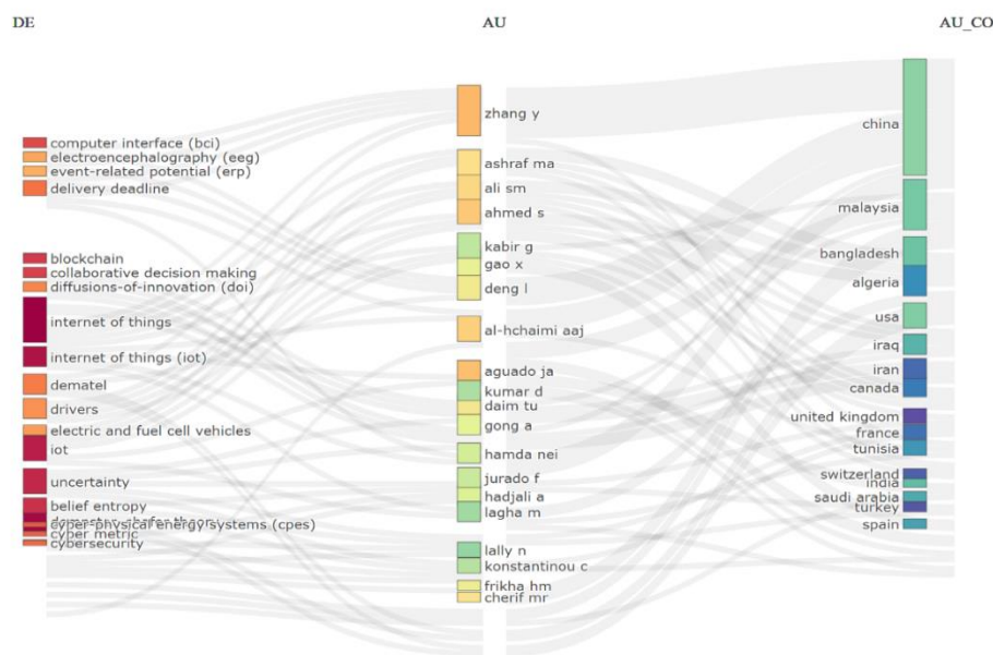
Fig. 2. Three-Field Plot
