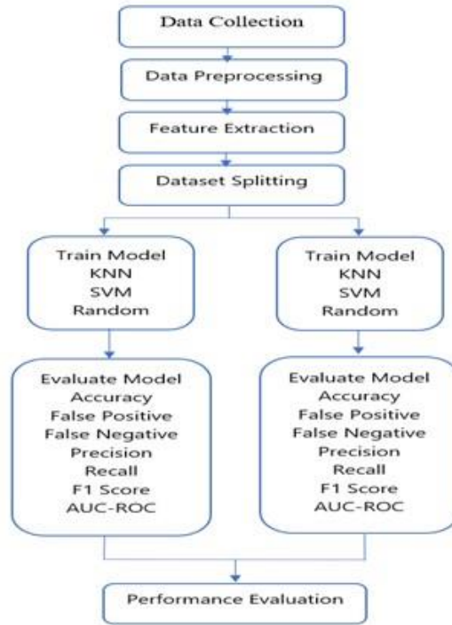
Fig. 5. Flowchart of the Machine Learning Process for DDoS Detection in IoT Networks
