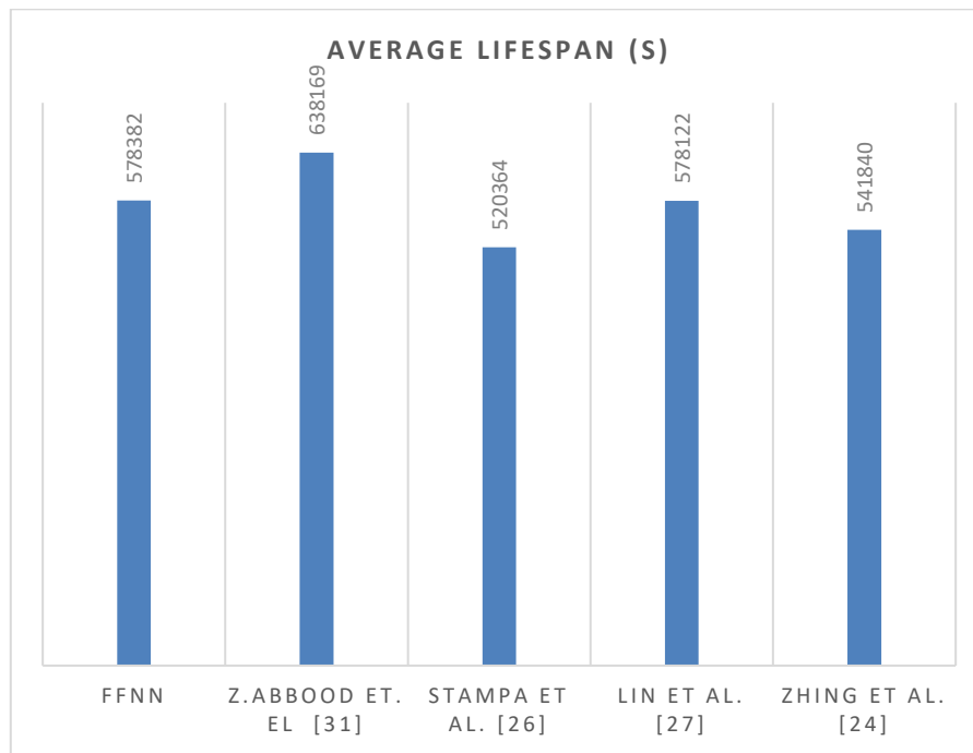
Fig. 9. Comparison of network lifespan across methods.
