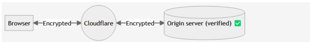
FIG. 9. FULL (STRICT) - SSL/TLS ENCRYPTION MODES
