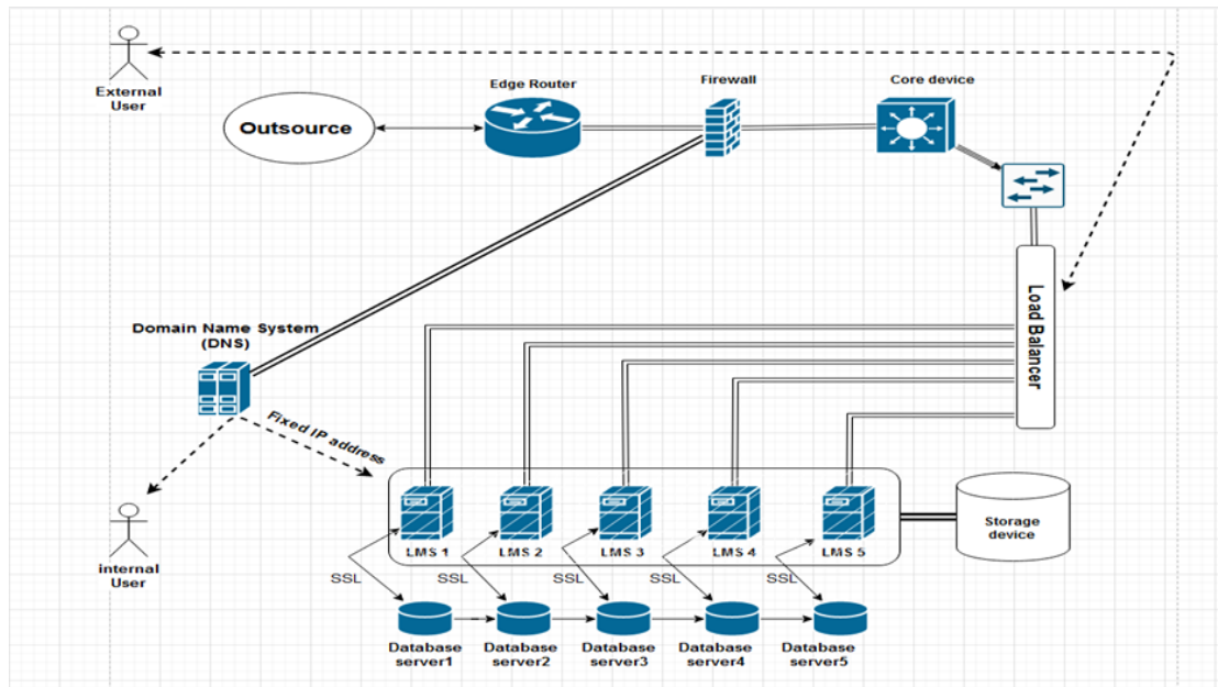
FIG.3. LMS INFRASTRUCTURE AT IUL
