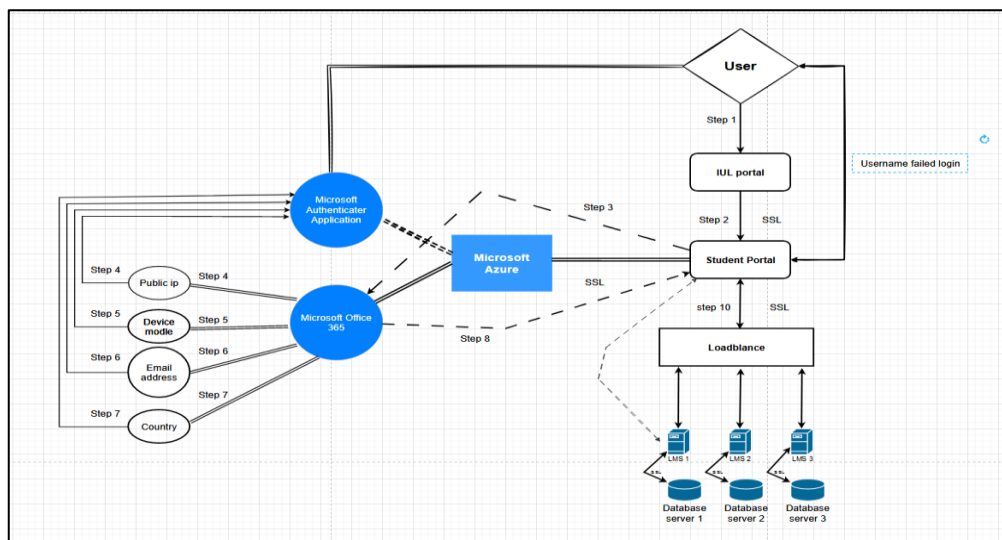
FIG.7. USER MOODLE PROCESS LOGIN BY MICROSOFT AZURE
