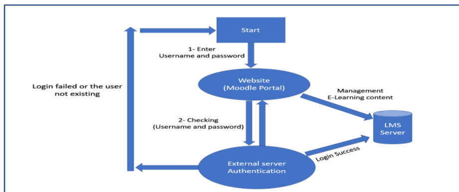
FIG. 19. FLOWCHART MOODLE INTEGRATION WITH EXTERNAL AUTHENTICATION SERVER
