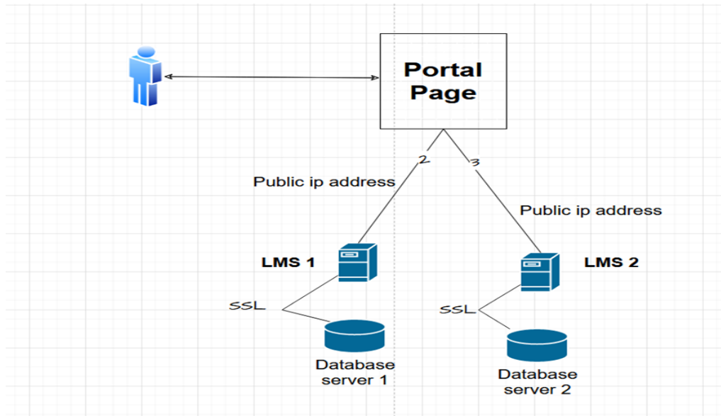
FIG. 6. MOODLE PROCESS FOR LOGIN AT IUL
