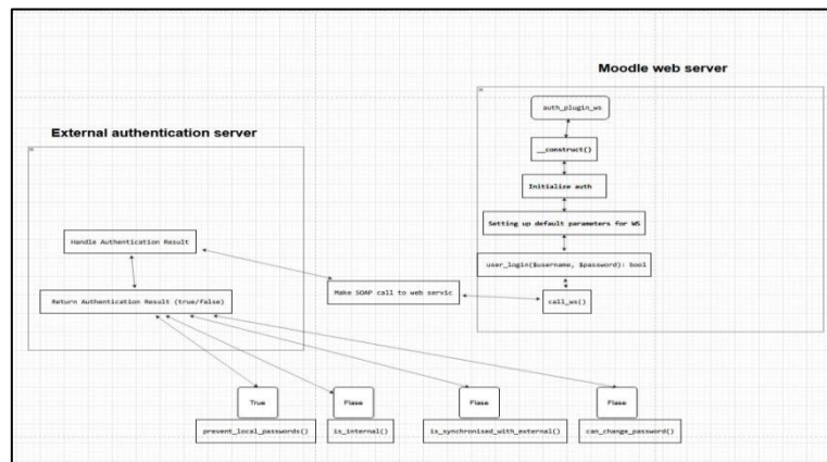
FIG. 20. A FLOWCHART TO VISUALIZE THE LOGIC OF THE (AUTH_PLUGIN_WS) CLASS.
