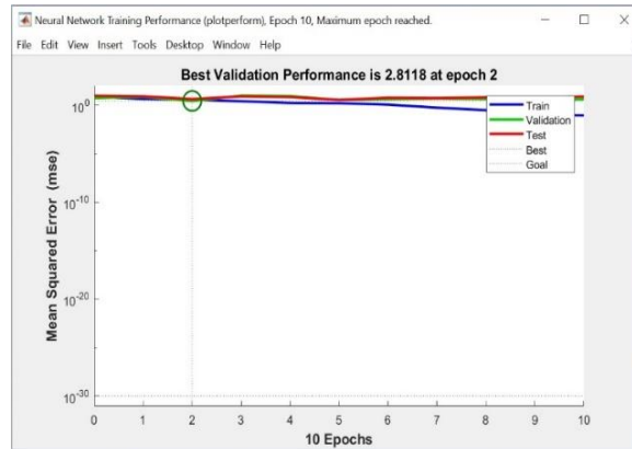
Fig. 15. Optimal algorithm performance validation target (MATLAB output).
