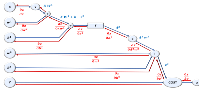
Fig. 7. Wight computation for convolutional neural network algorithms.
