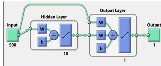
Fig. 9. The FFNN algorithm's design.
