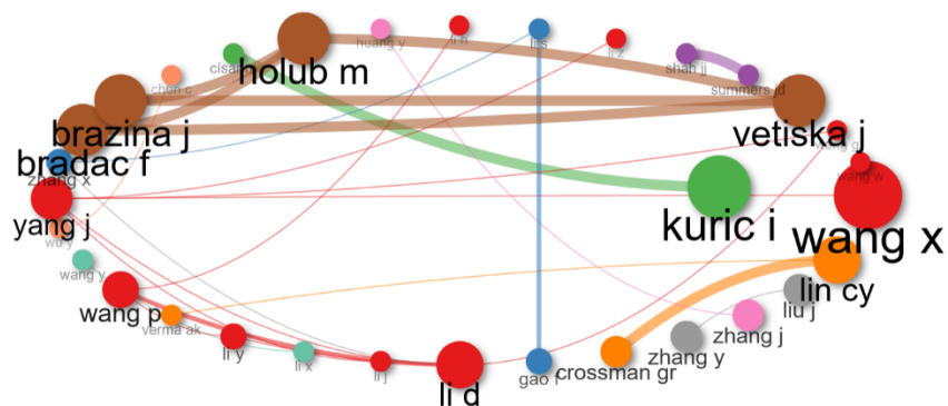
Fig. 6. Visualization of Collaboration Network
