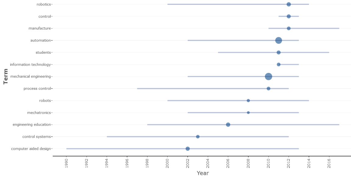
Fig. 5. Visualization of Trend Topics
