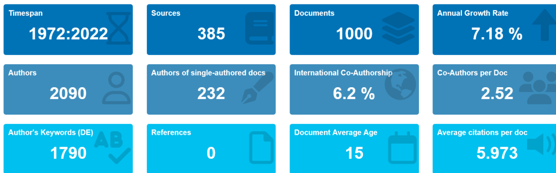
Fig. 1. Visualization of Key Insights from the Bibliometric Analysis
