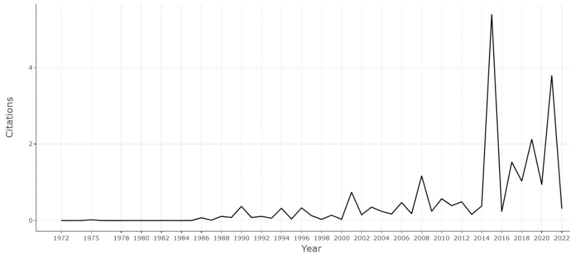
Fig. 3. Visualization of Average Citations per Year
