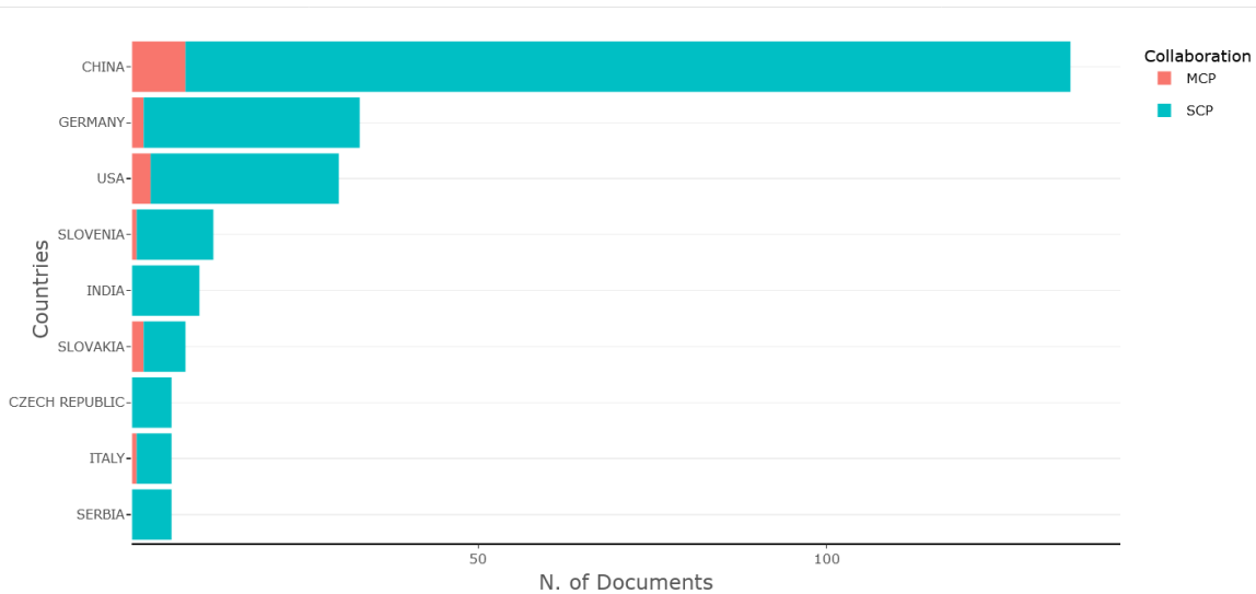
Fig. 4. Visualization of Corresponding Author's Countries
