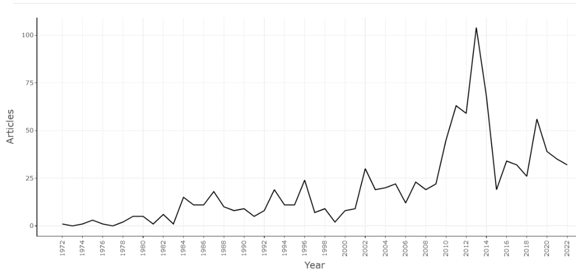
Fig. 2. Visualization of Annual Scientific Production
