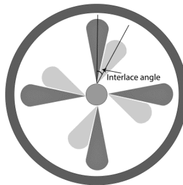
Fig. 6. Schematic of the dual-fuel DI concentric injector jet configuration on the top-plane[35].
