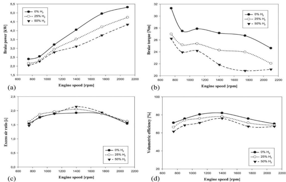
Fig. 7. (a) Variation of brake power, (b) brake torque, (c) excess air ratio (d) and volumetric efficiency depending on engine speed and hydrogen rate[93].
