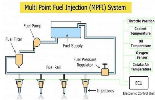
Fig. 2. Multi-Point Injection[37]
