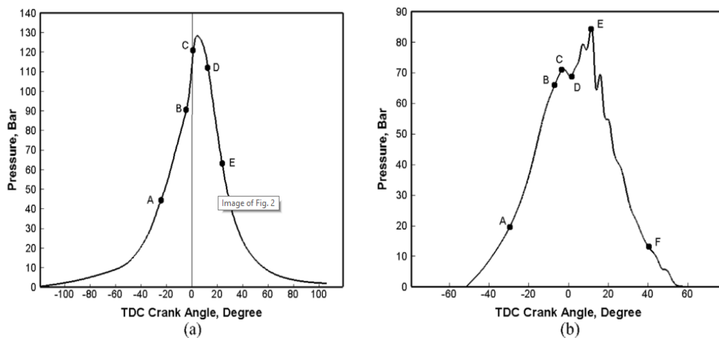
Fig. 4. Combustion process, (a) For diesel engine, and (b) For dual-fuel diesel engine [87].
