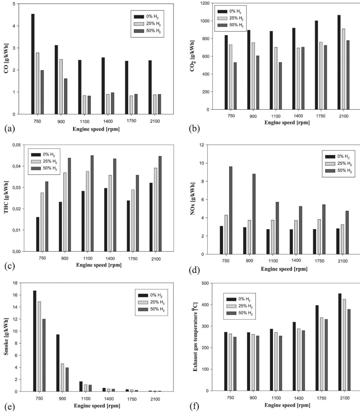
Fig. 9. (a) CO emission value variation, (b) CO 2 emission value variation, (c) THC emission value variation, (d) NO x emission value variation, (e) Smoke emission value variation and (f) exhaust gas temperature value variation based on engine speed at different hydrogen quantities[93].
