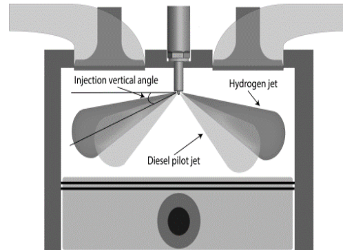
Fig. 5. Schematic of the dual-fuel DI concentric injector jet configuration on the axial cross-sectional plane[35].
