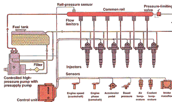
Fig. 3. Common Rail Direct Injection[44]
