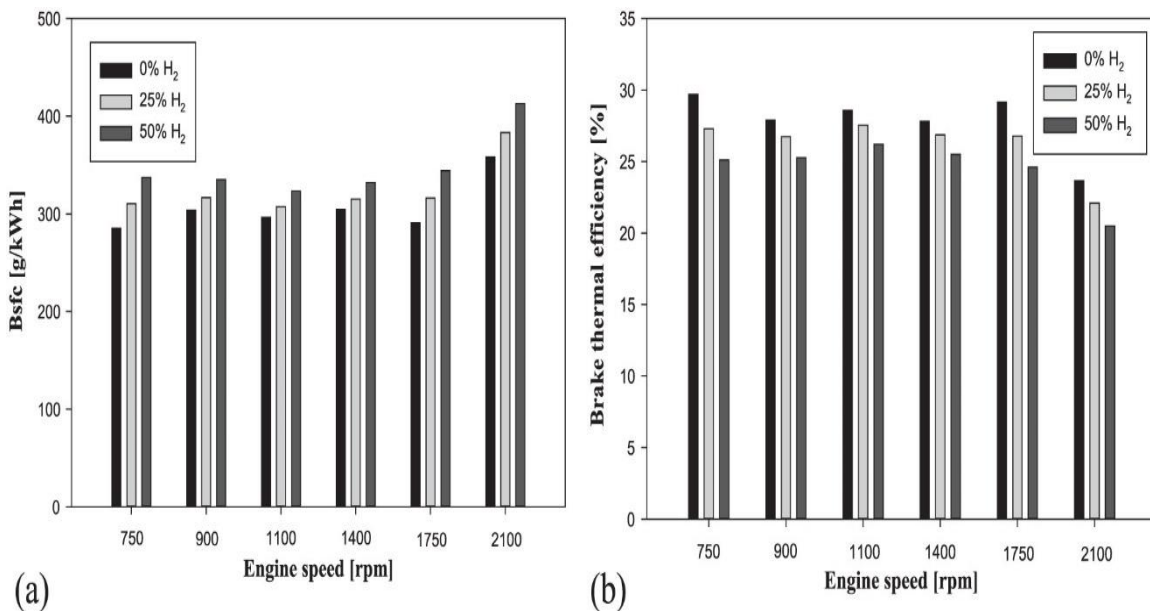
Fig. 8. (a) Brake-specific fuel consumption value variation at different hydrogen quantities based on engine speed and (b) brake thermal efficiency value variation at different hydrogen quantities based on engine speed[88,92].
