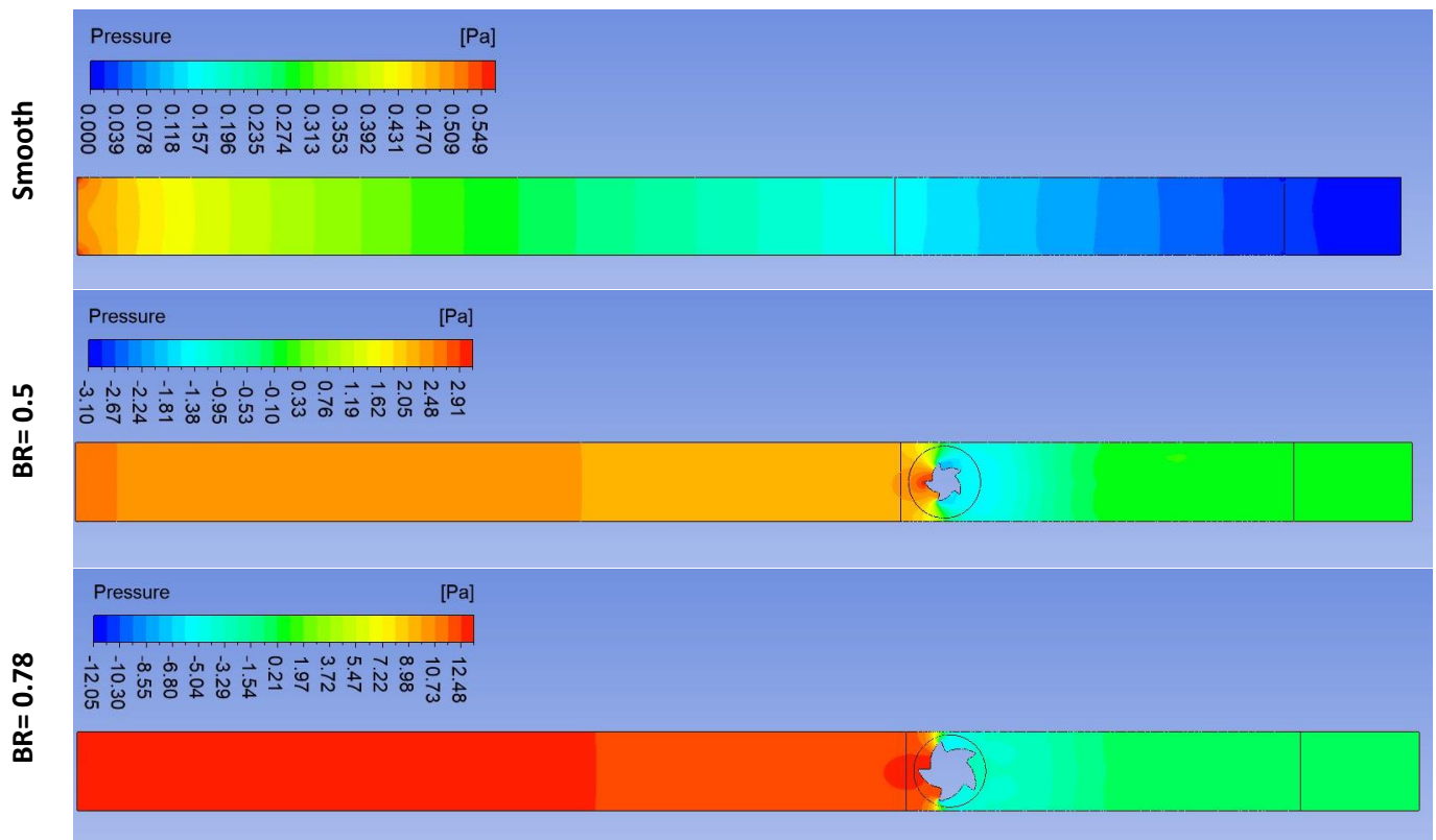
Fig. 9. Pressure distribution
