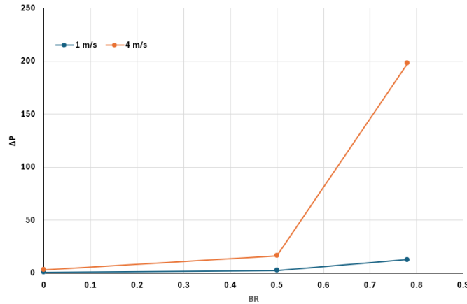
Fig. 7. Effect of velocity and blocking ratio on pressure drop.
