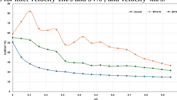
Fig. 4. Local heat transfer coefficient for different blocking ratios ( V = 1\text{m/s} ).
