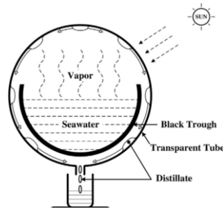
Fig.1. A tubular solar still
