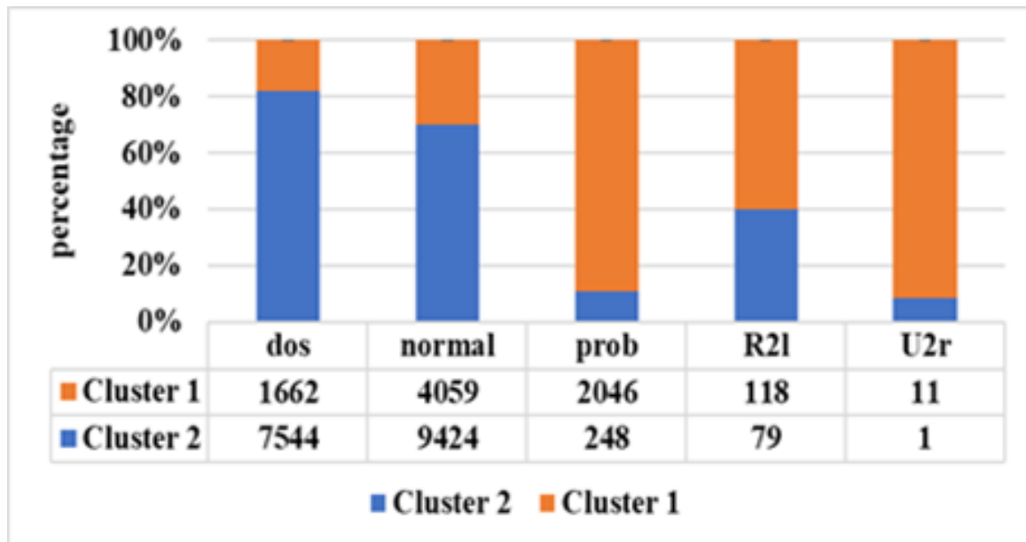
(a) full features of NSL-KDD Data Clusters.
