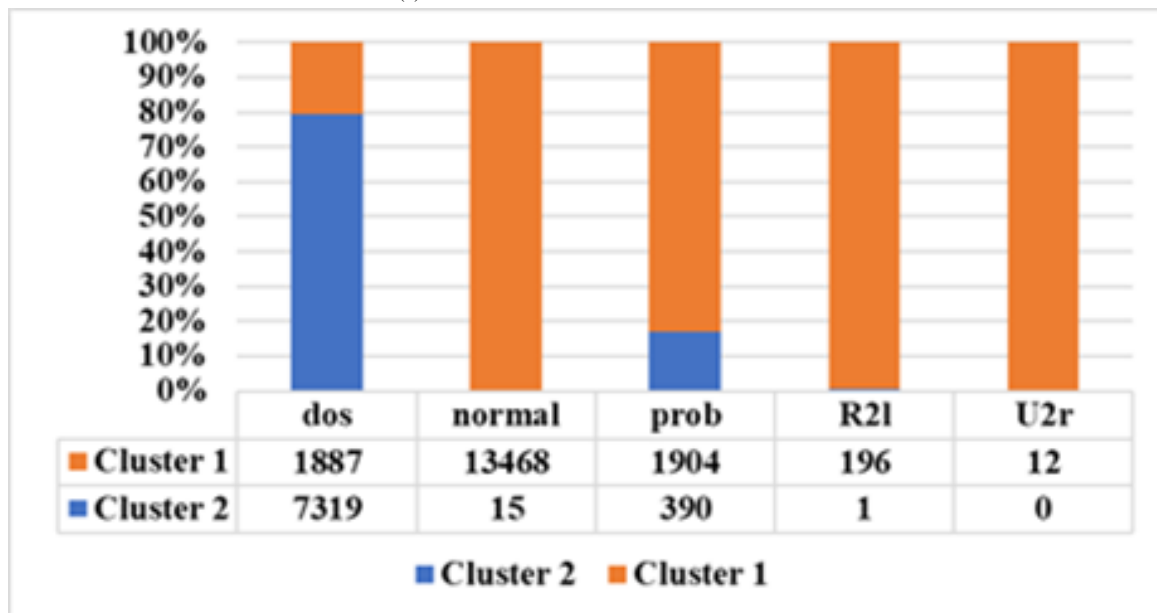
(b) 94 Features Of NSL-KDD Data Clusters.
