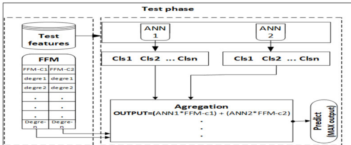
Fig. 2. Illustrates The Aggregation Method Predict Final Output.
