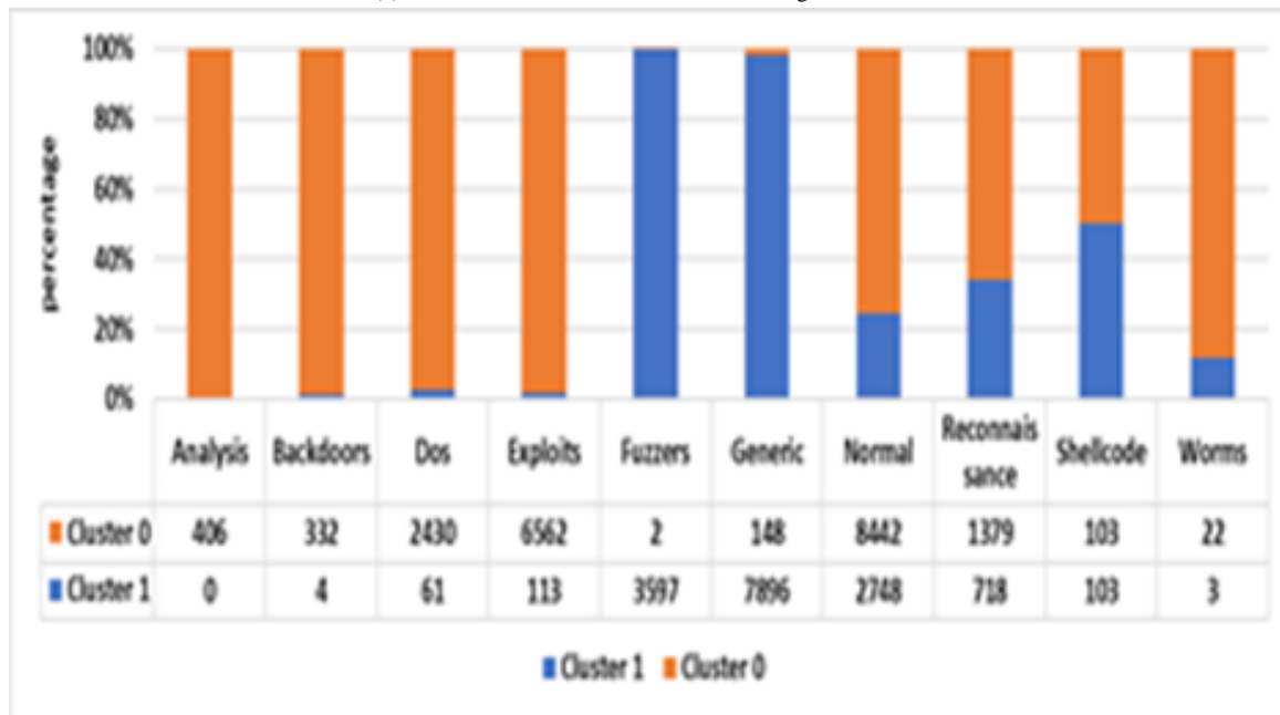
(b) 158 Features Of UNSW-NB15 Data Clusters.
