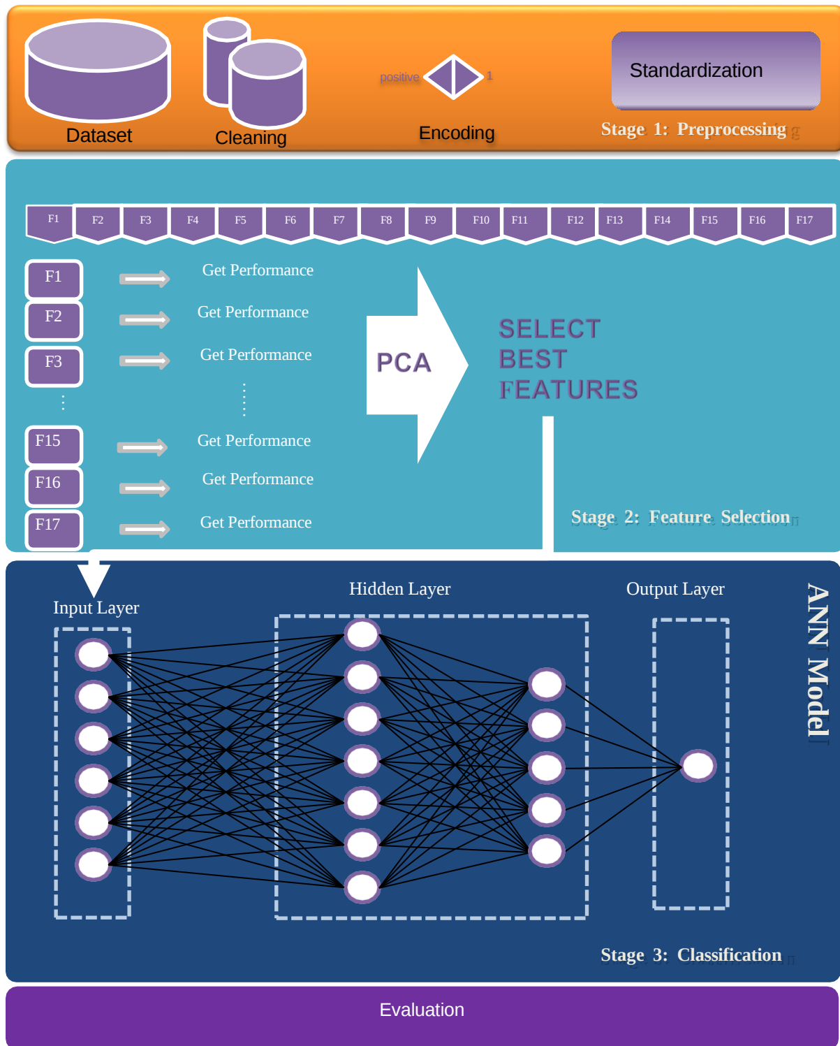
Fig. 1. Research Methodology
