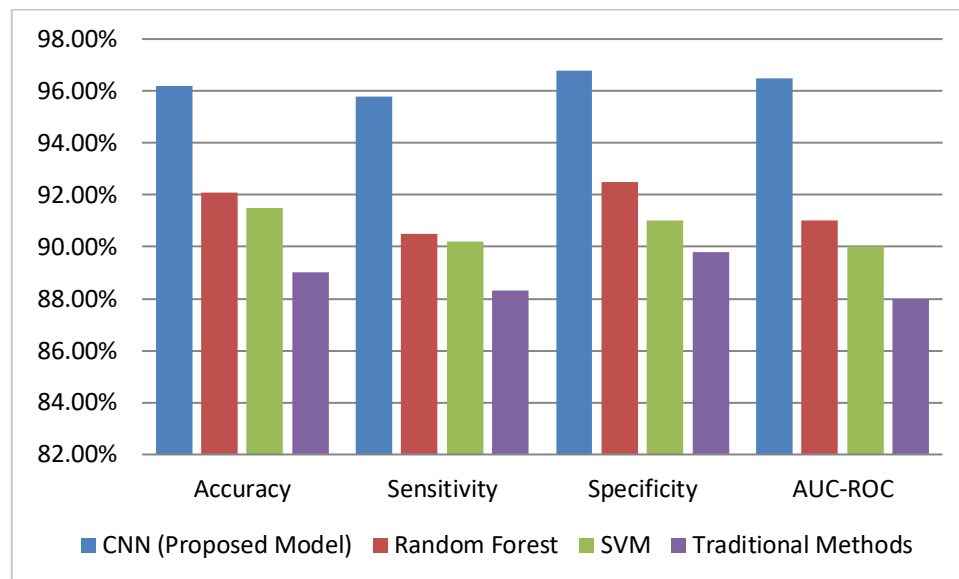
Fig. 2. presents a comparative analysis of four machine learning models—CNN (Proposed Model), Random Forest, SVM, and Traditional Methods—evaluated on four key performance metrics: Accuracy, Sensitivity, Specificity, and AUC-ROC.
