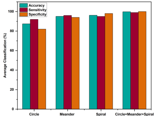
Fig. 3. Results were obtained after extracting features using VGG16.
