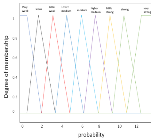
Fig.12. Likelihood of LEACH-FL
