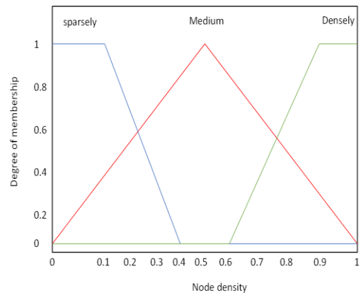
Fig.10. Node density in LEACH-FL
