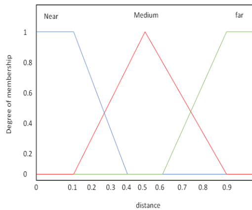
Fig.9. LEACH-FL Distance
