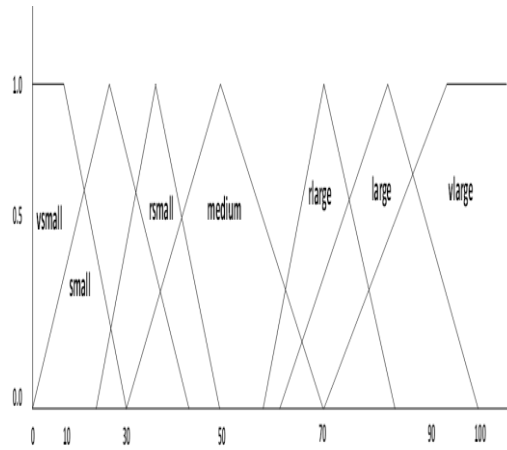
Fig.7. potential application of Gupta's Fuzzy Logic
