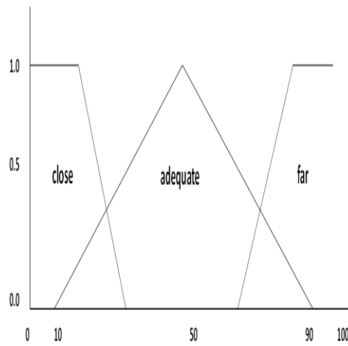
Fig.6. Gupta's Fuzzy Logic Centralization
