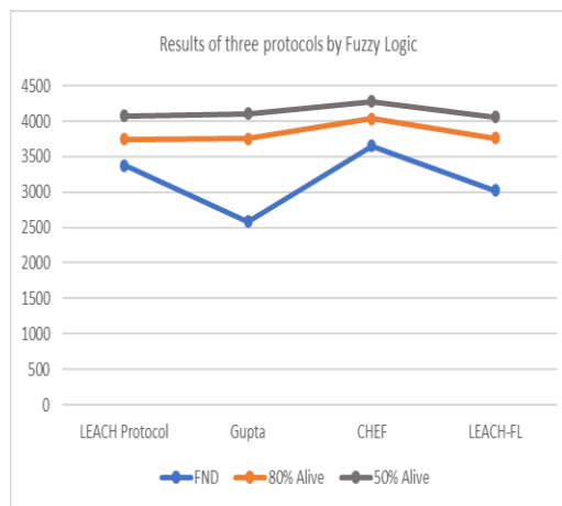
Fig.14. Three protocols via Fuzzy Logic
