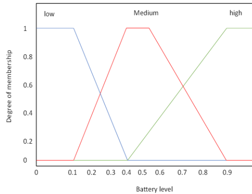
Fig.11. The battery life of LEACH-FL
