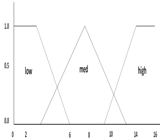
Fig.5. Gupta's Fuzzy Logic concentration metrics
