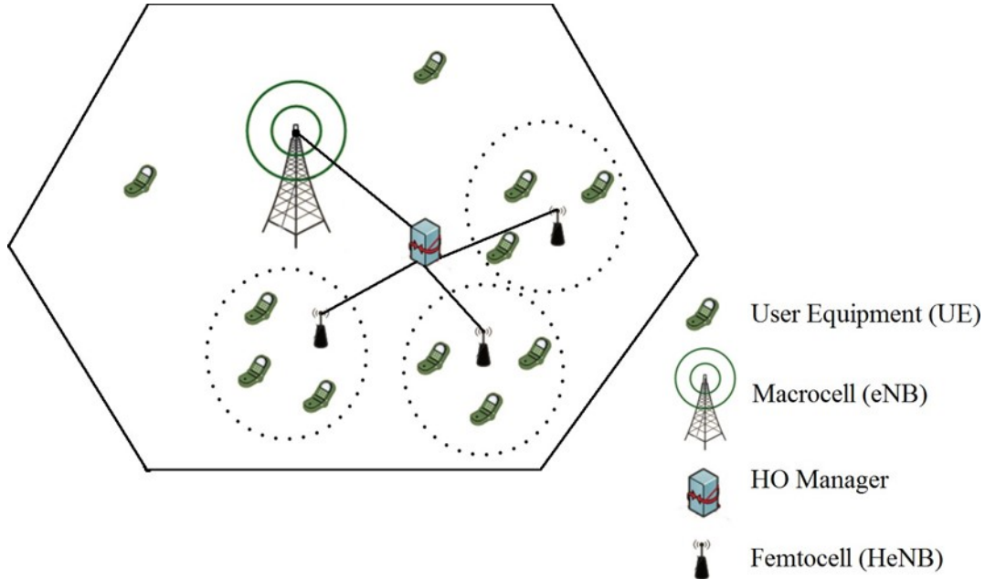
Fig. 3. network topology [11]
