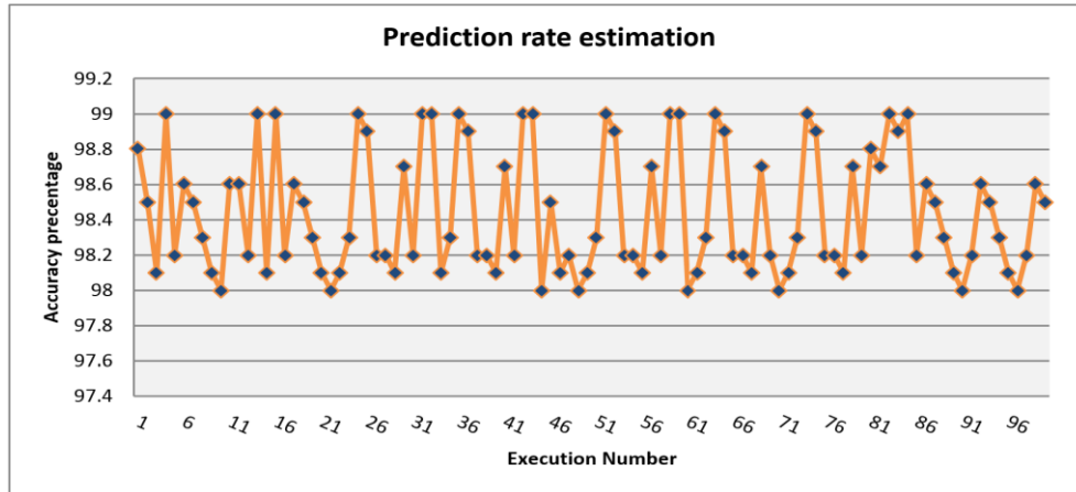
Fig. 13. Proposed system prediction estimation.
