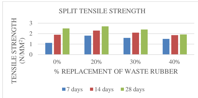
Fig.3. Split Tensile Strength
