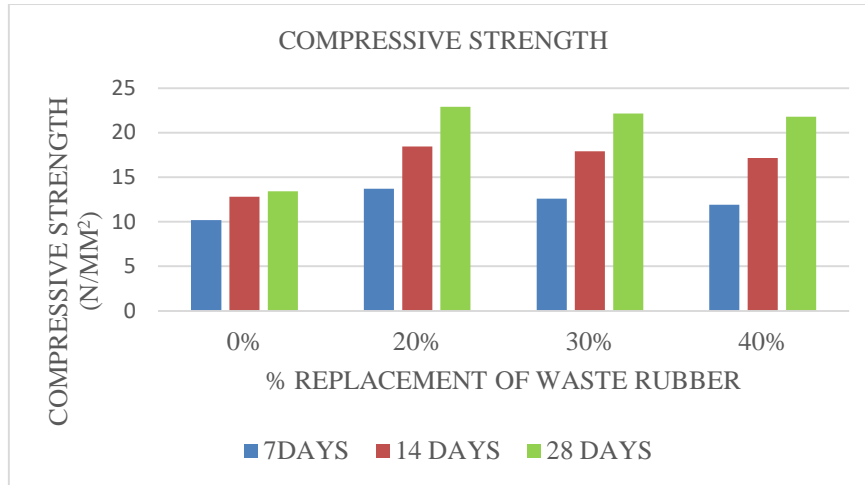
Fig.1. Compressive Strength
