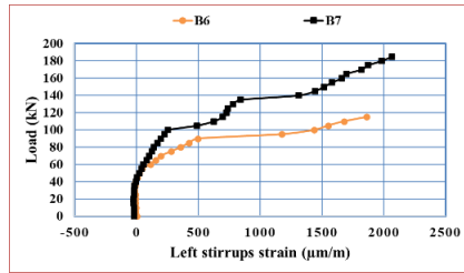
a. Left side stirrups strain for beams B6 and B7 .
