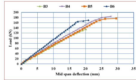
Load deflection curves of beams B1, B2 and load deflection curves of beams B3, B4, B5 and B6
