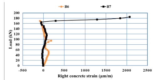
b. Right side concrete strain for beams B6 and B7 .
